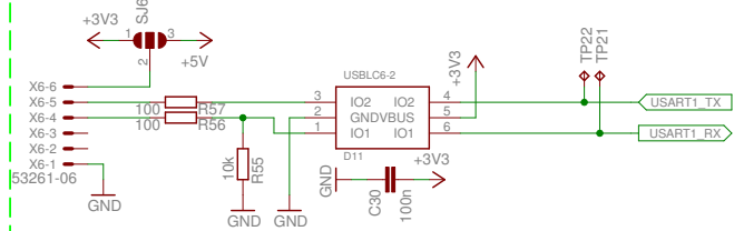
General Purpose UART1
