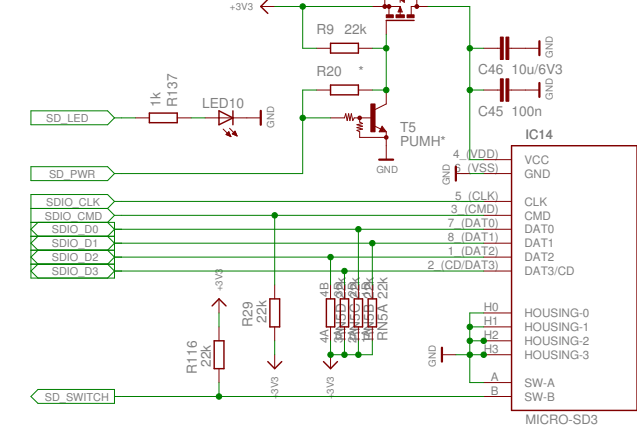
"microSD" card interface
