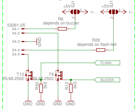
Buzzer & Flashlight
