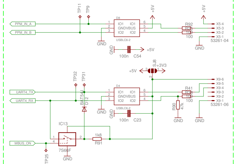
PPM - Receiver Ports & RS232 / MBUS Interface (USART4)
