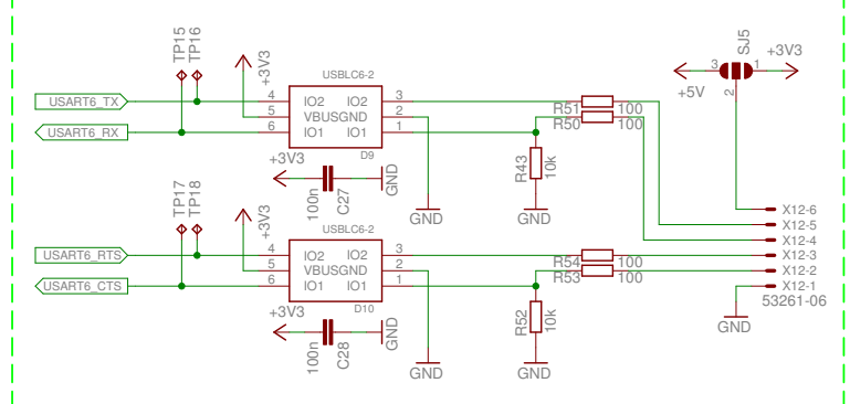
General Purpose UART6 (Modem and High-Speed capability)
