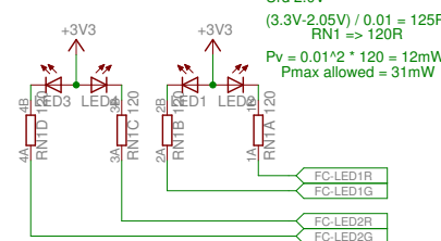
FC-Status LEDs
