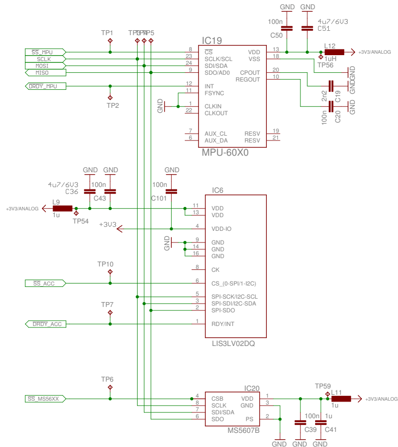
ACC, Gyro, Pressure & Temperature- Sensor, Channel A
