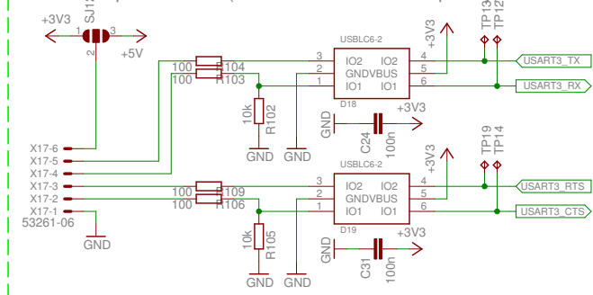
General Purpose UART3 (Modem and bootloader capability)
