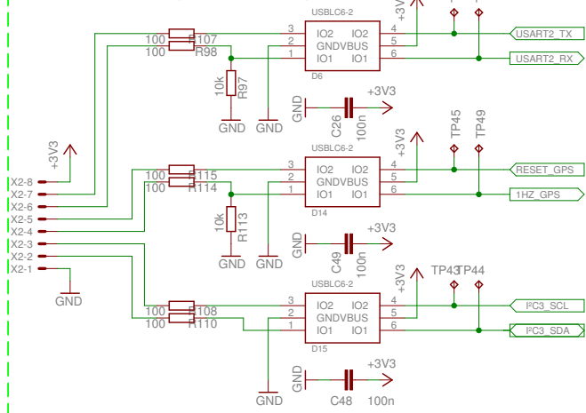
GPS & KOMPASS ( UART2 & I2C3 )
